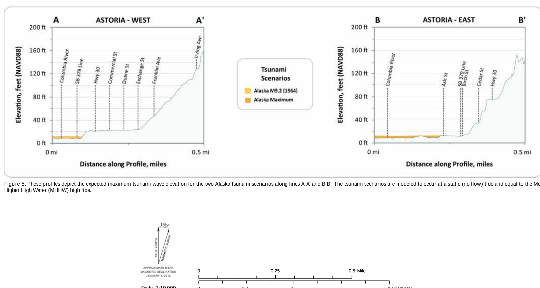
Figure 5: These profiles depict the expected maximum tsunami wave elevation for the two Alaska tsunami scenarios along lines A-A' and B-B'. The tsunami scenarios are modeled to occur at a static (no flow) tide and equal to the Mean Higher High Water (MHHW) high tide.
