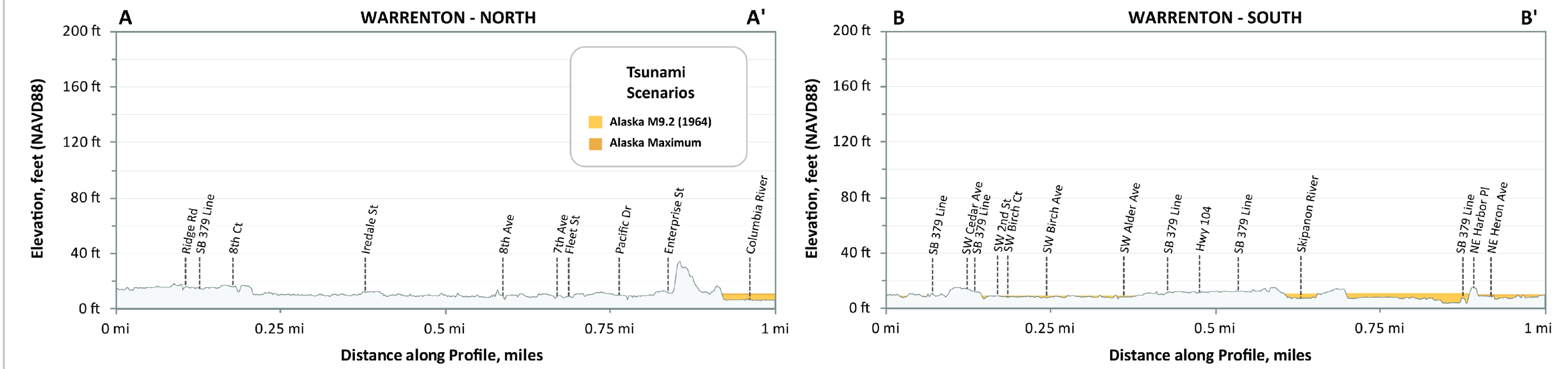
Figure 5: These profiles depict the expected maximum tsunami wave elevation for the two Alaska tsunami scenarios along lines A-A' and B-B'. The tsunami scenarios are modeled to occur at a static (no flow) tide and equal to the Mean Higher High Water (MHHW) high tide.
