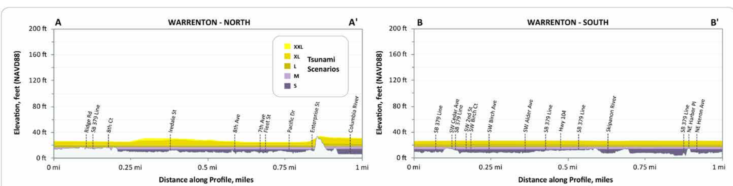
Figure 6: These profiles depict the expected maximum tsunami wave elevation for the five "T-shirt" scenarios along lines A-A' and B-B'. The tsunami scenarios are modeled to occur at high tide and to account for local subsidence or uplift of the ground surface.
