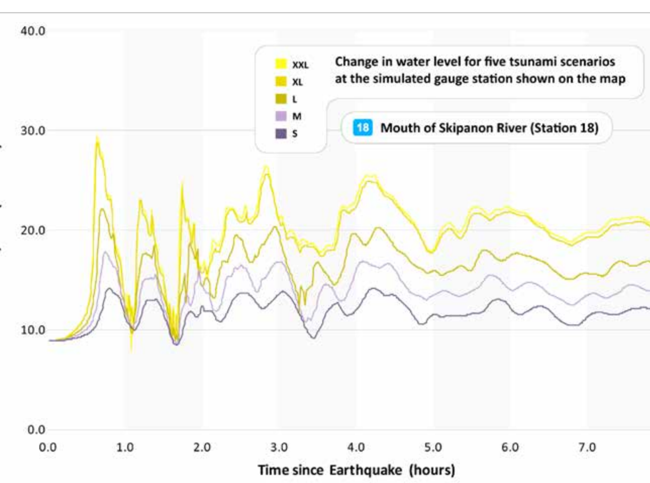
Figure 5: This chart depicts the tsunami waves as they arrive at the selected reference point (simulated gauge station). It shows the change in wave heights for all five tsunami scenarios over an 8-hour period. The starting water elevation (0.0 hour) takes into account the local land subsidence or uplift caused by the earthquake. Wave heights vary throughout time, and the first wave will not necessarily be the largest as waves interact and reflect off local topography and bathymetry. Any absence of data indicates periods for which tsunami inundation has not yet reached or has receded from the station location and dry land is exposed.
