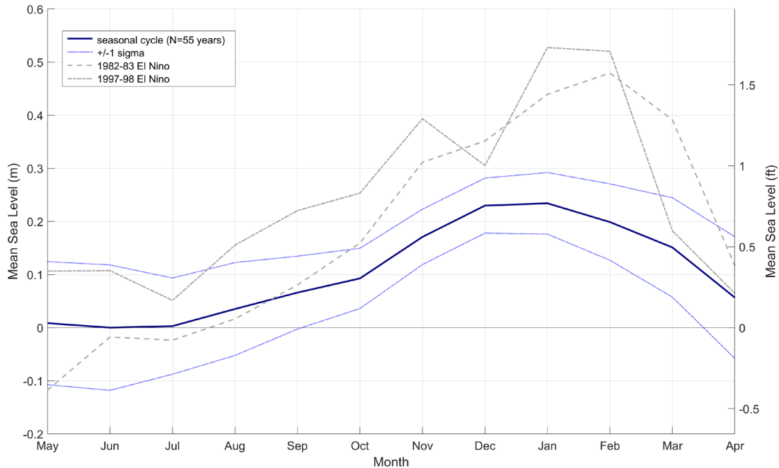
Figure 4-3. Seasonal cycles in monthly mean water levels based on data from the South Beach tide gauge (1967-2022). Data from National Ocean Service.
