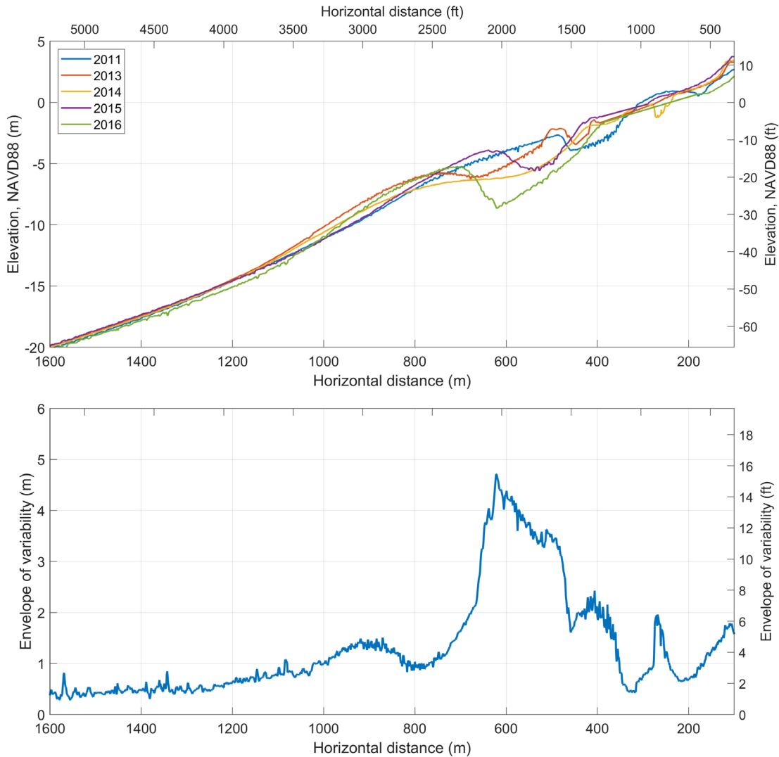
Figure 4-7. Repeat topo-bathymetric surveys performed at line 053, Rockaway Beach, Oregon. Top plots depict the serial beach and nearshore profile surveys and the bottom plot shows the envelope of variability determined from all surveys. Data from Allan and others (2015d) and Cohn and others (2019).
