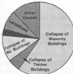
EARTHQUAKE FATALITIES 1950 - 1990
