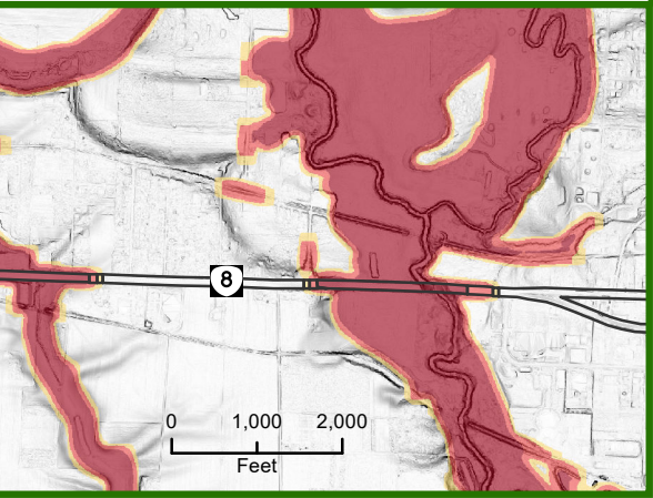
Closeup, Oregon Highway 8, showing potential permanent ground deformation (same color scale as main map)
