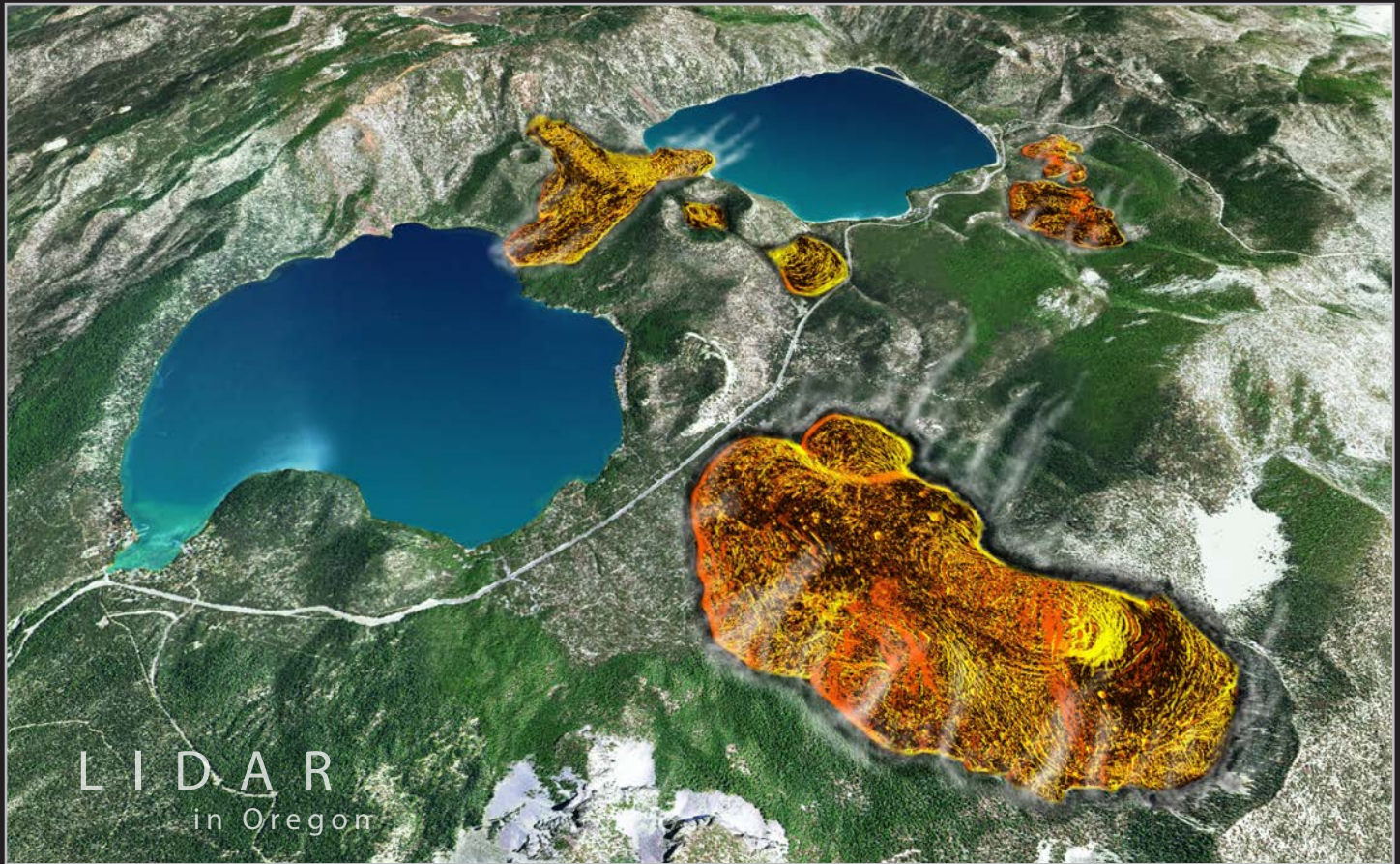
Big Obsidian Flow and Other Major Lava Flows, Newberry Crater, Oregon
