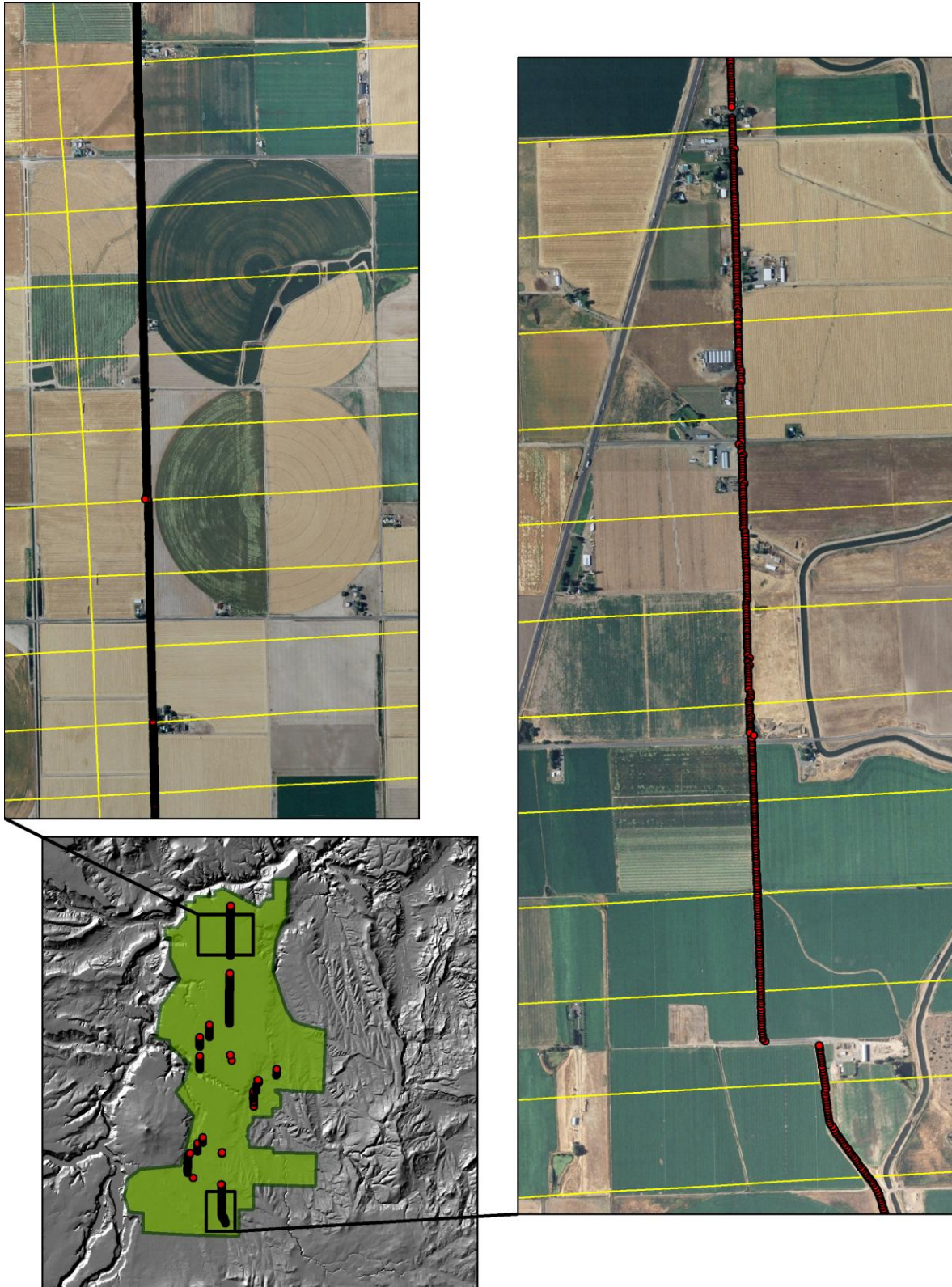
Figure 2.16. Selected RTK point locations in the study area for the current delivery, area 17; images are NAIP orthophotos.
