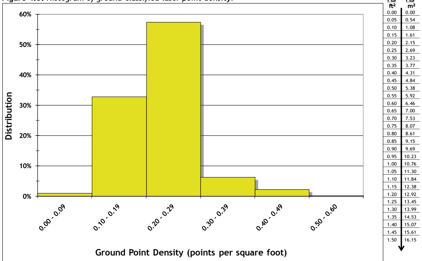
Figure 4.3. Histogram of ground-classified laser point density.
