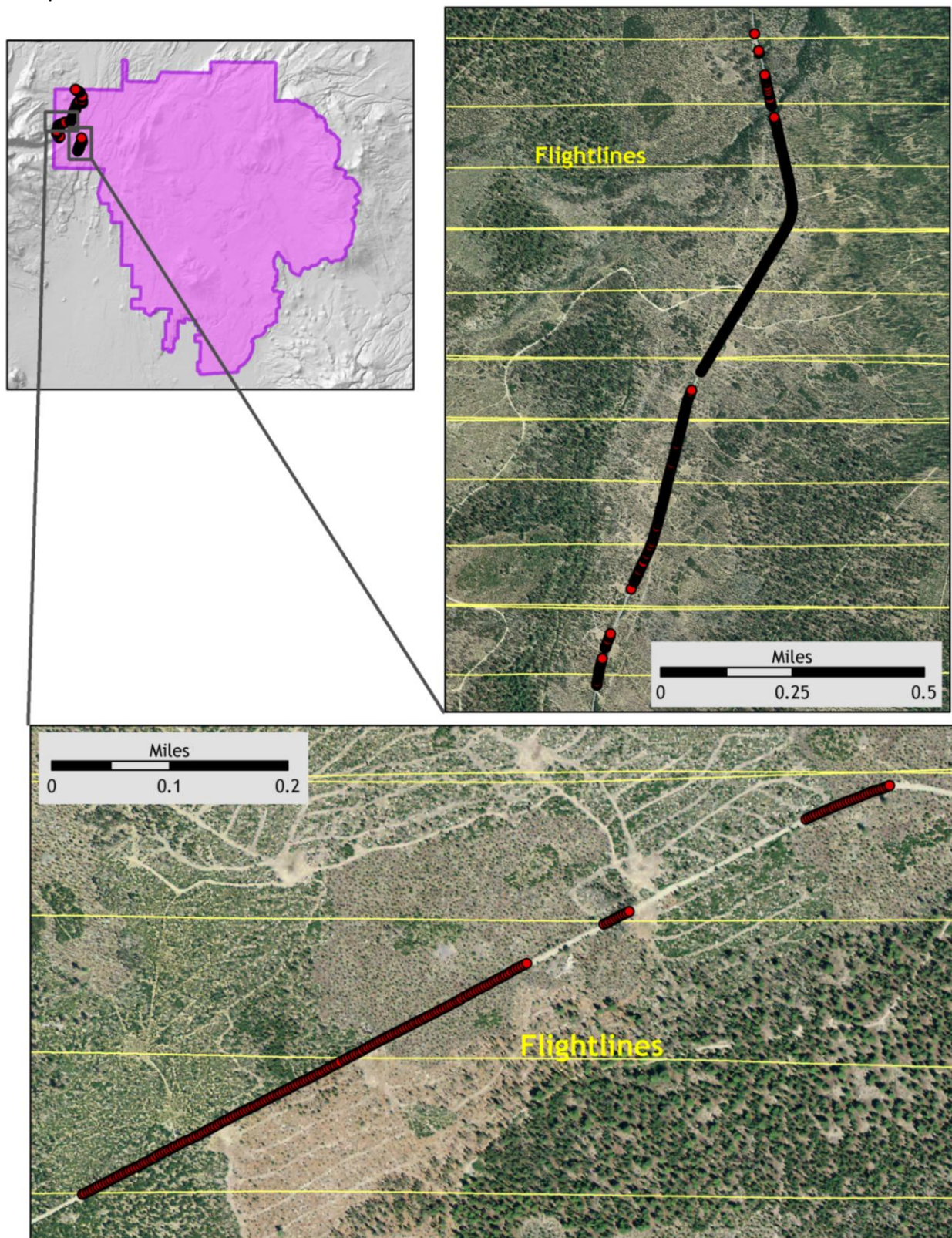
Figure 2.14. Selected RTK point locations in the study area for delivery area 13; images are NAIP orthophotos.
