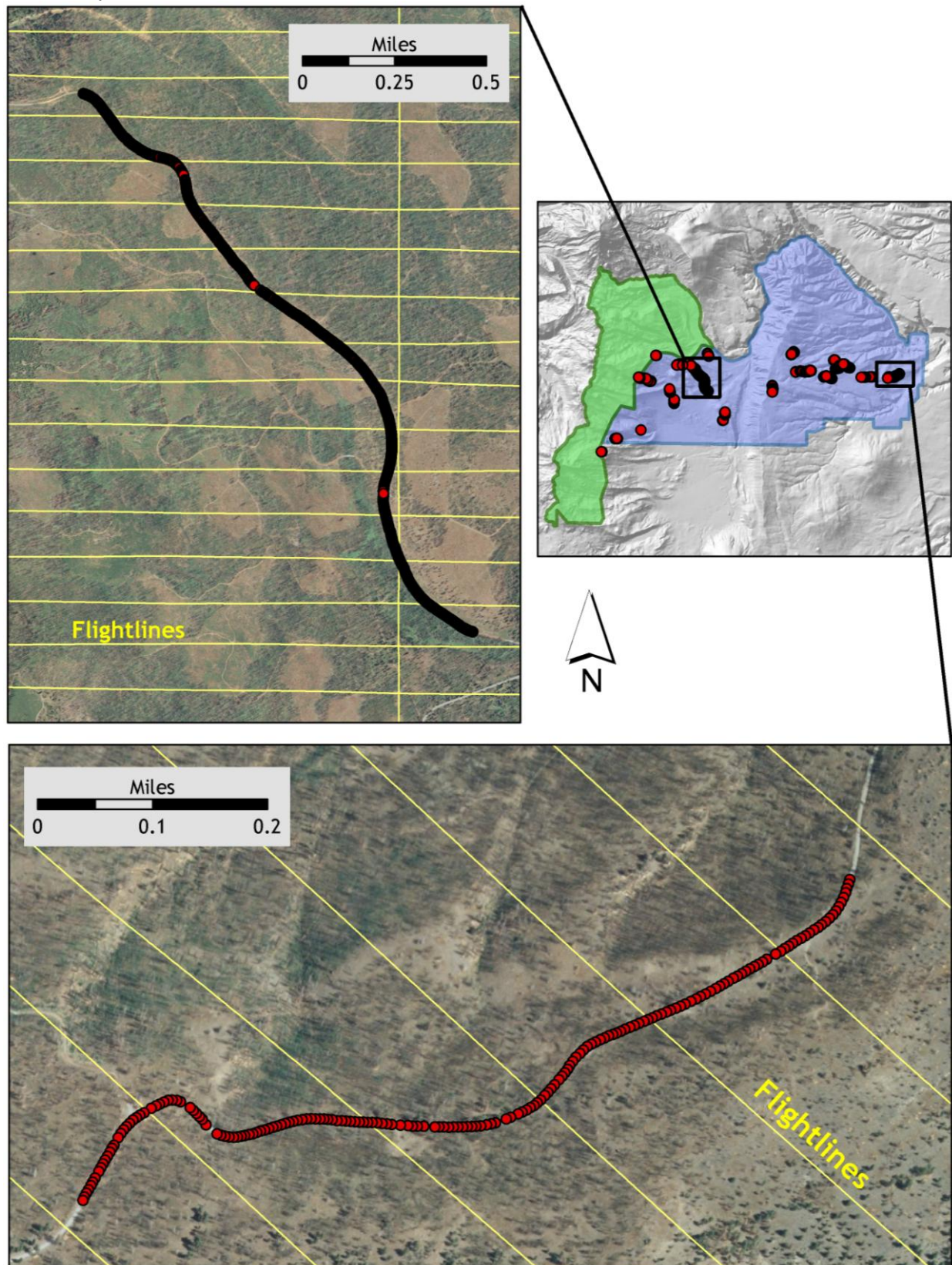
Figure 2.4. Selected RTK point locations in the study area for delivery areas 2 and 14; images are NAIP orthophotos.
