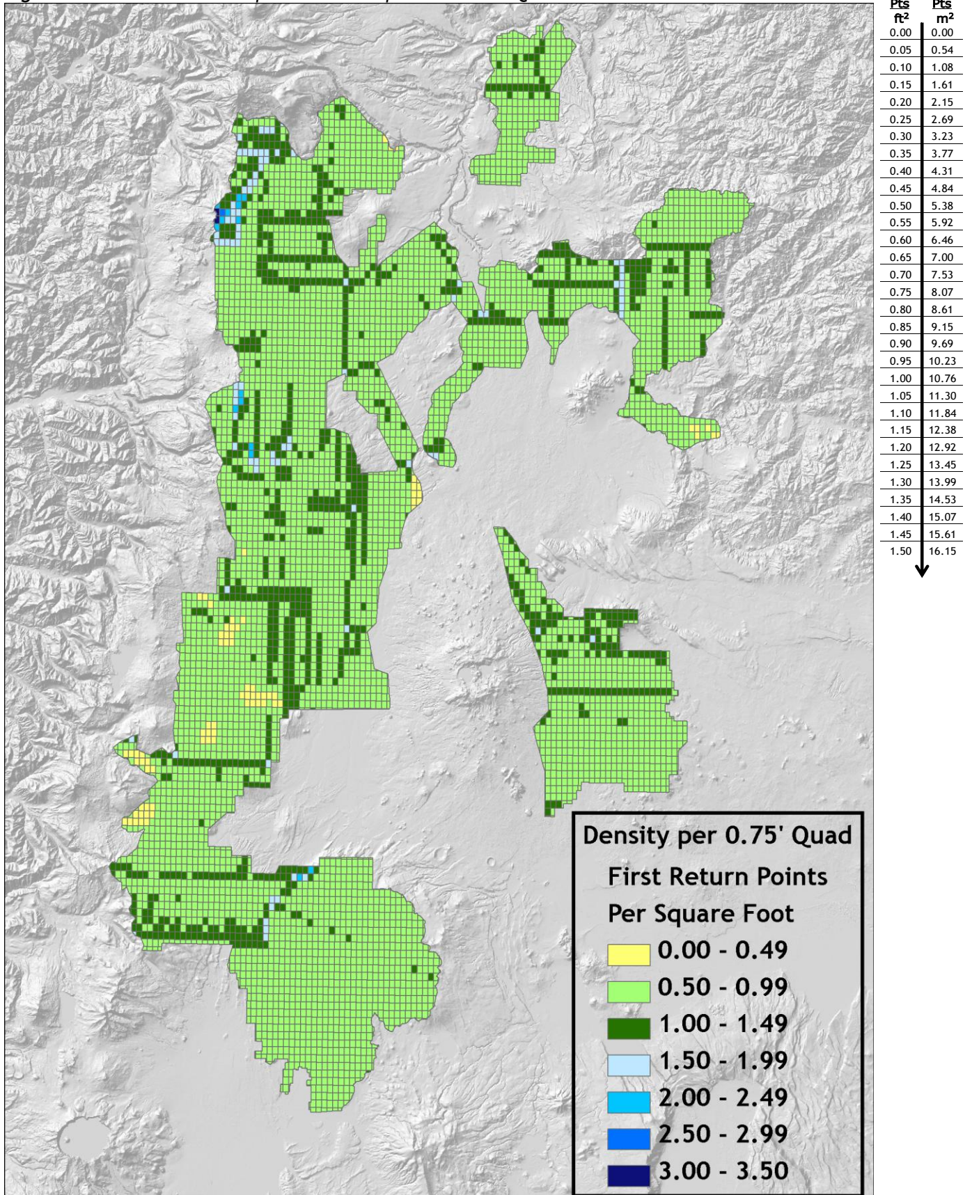
Figure 4.2. First return laser point densities per 0.75' USGS Quad.
