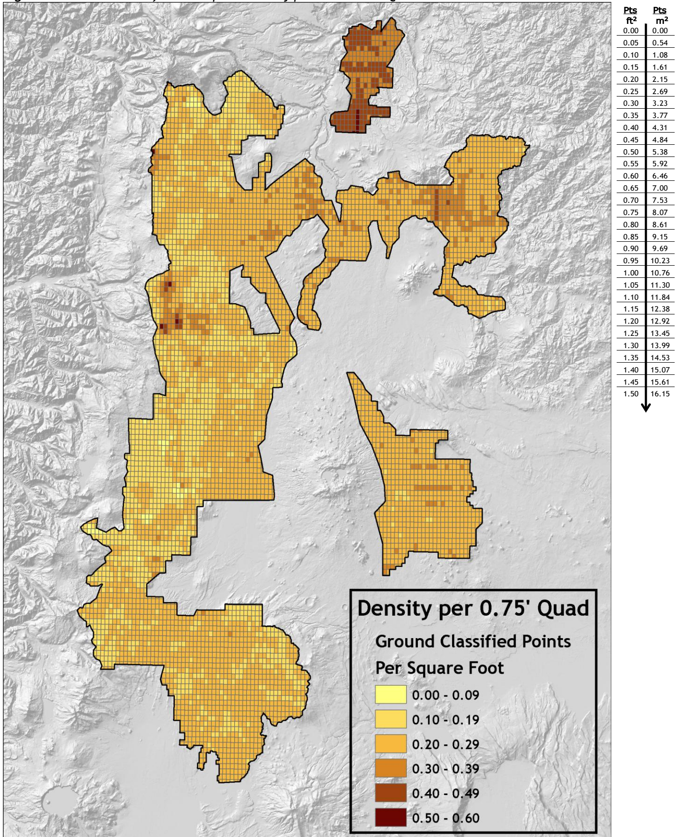
Figure 4.4. Ground-classified laser point density per 0.75' USGS Quad.
