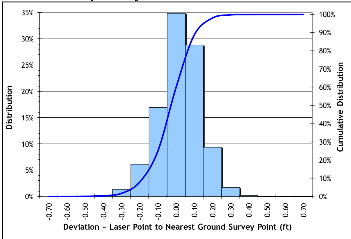
Figure 3.3. Deschutes Study Area histogram statistics
