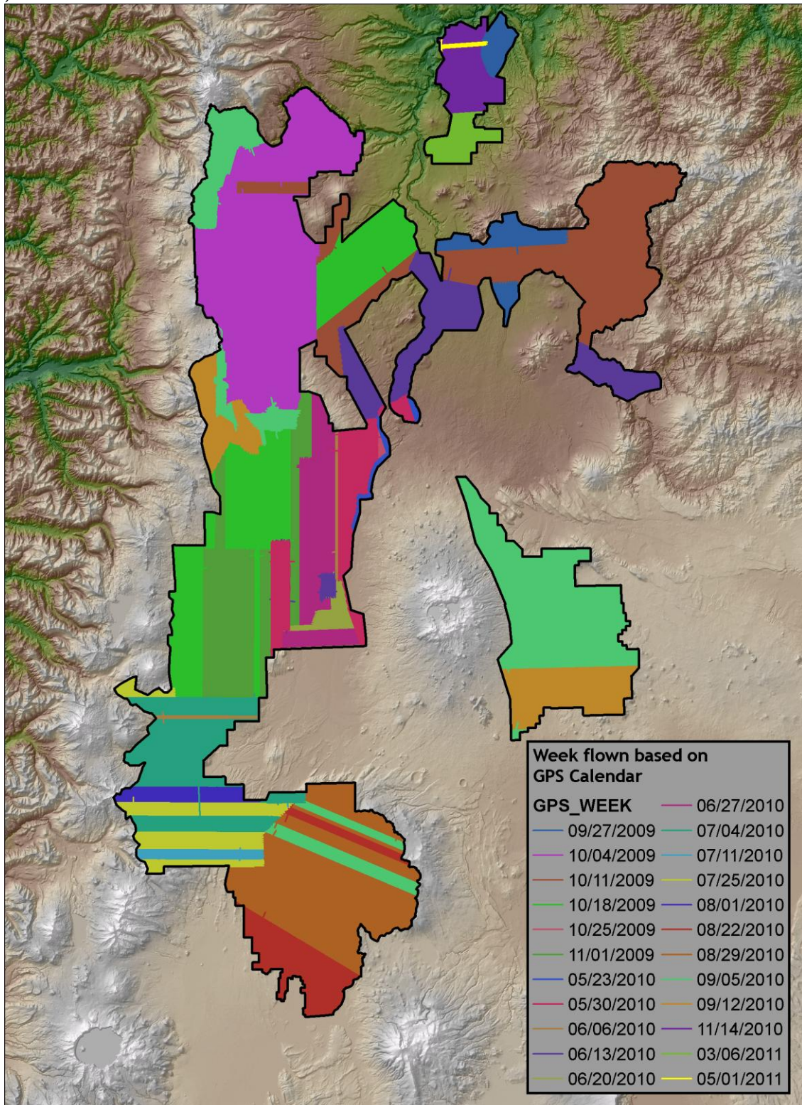
Figure 2.1. Actual flightlines for the Deschutes Study Area illustrating the dates flown (based on GPS week).
