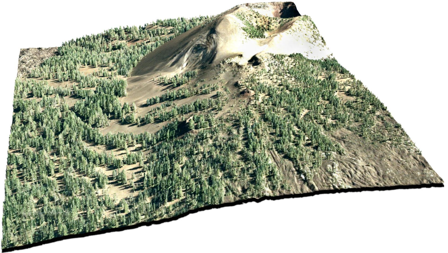
Belknap Crater, viewed from the southwest. Image created from LiDAR point cloud with RGB values extracted from NAIP orthophoto.
