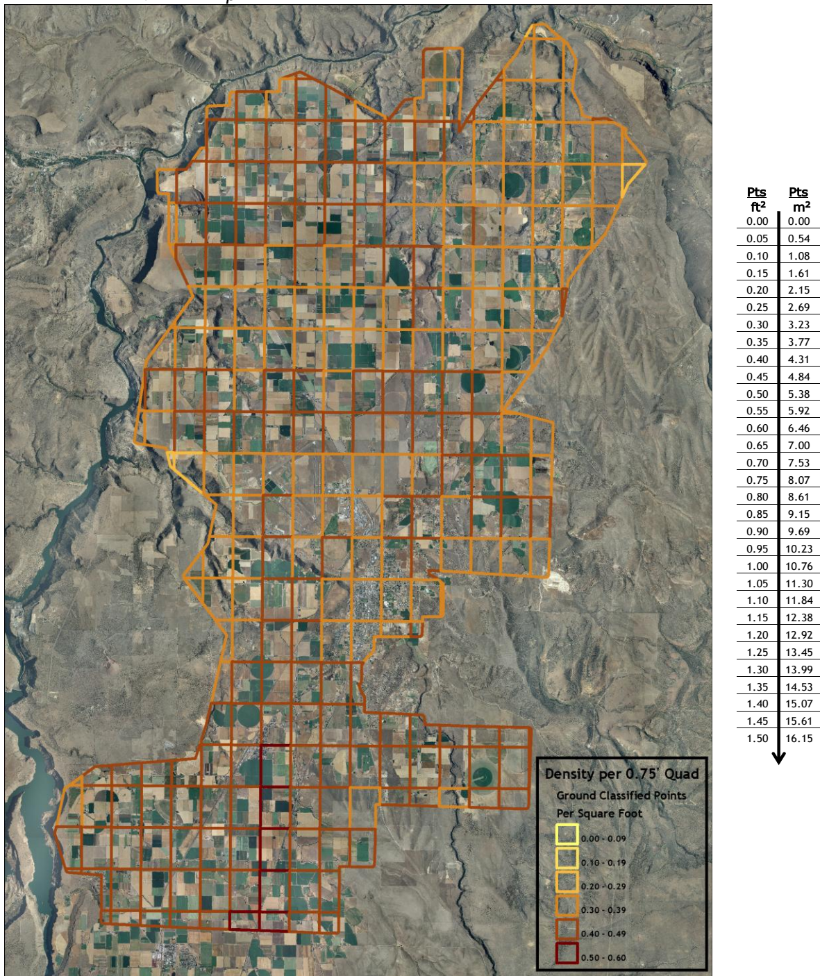
Figure 4.5. Ground-classified point density in delivery areas 1 and 17 of the Deschutes study area overlaid onto a NAIP orthophoto.
