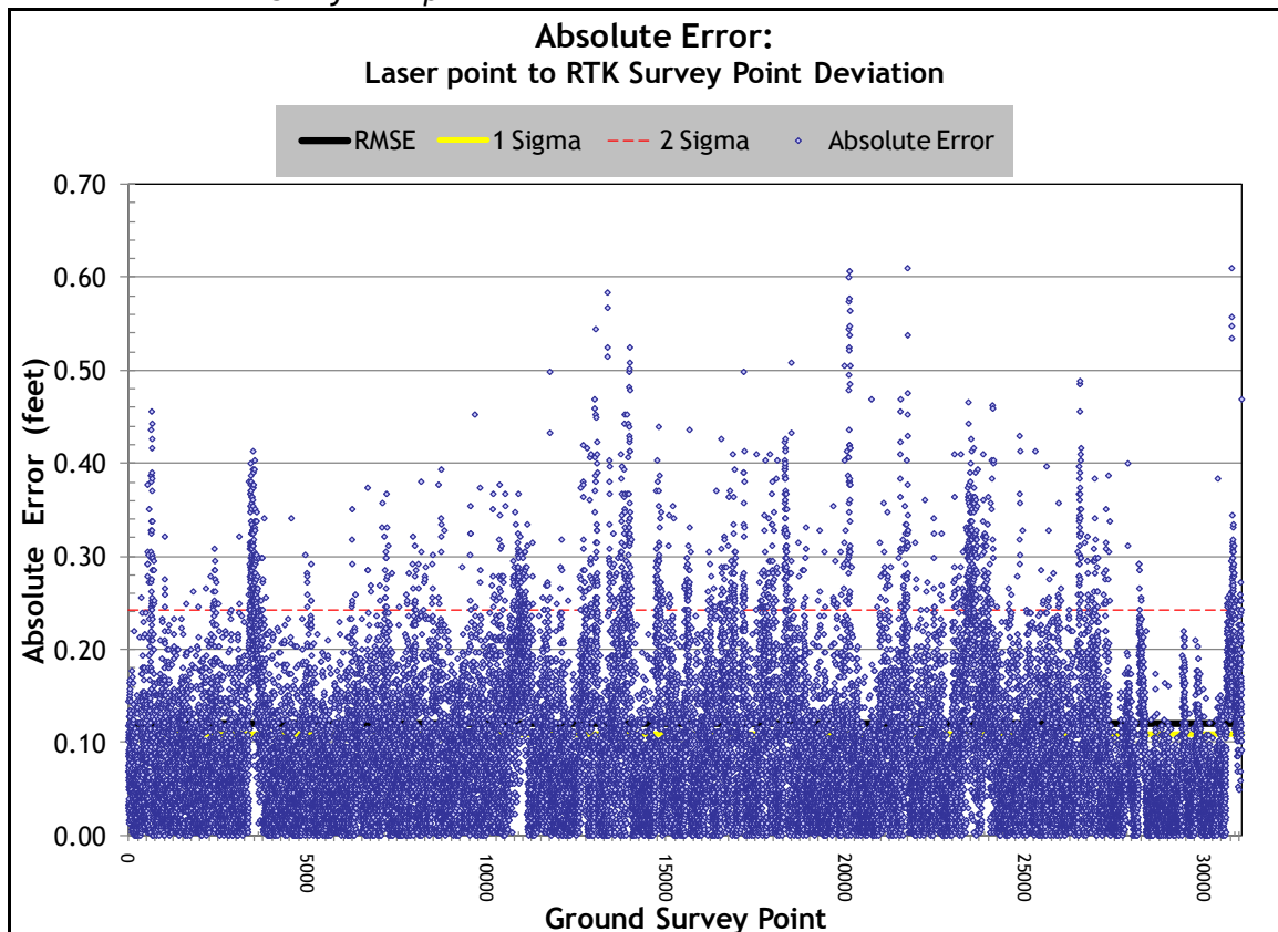
Figure 3.4. Deschutes Study Area point absolute deviation statistics.
