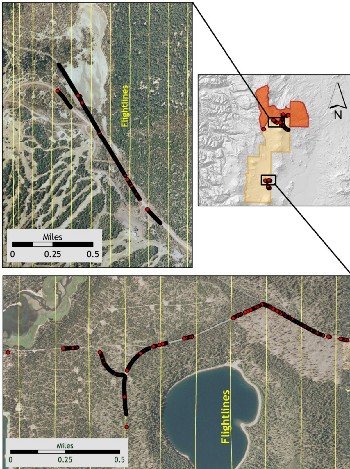
Figure 2.8. Selected RTK point locations in the study area for delivery areas 7 and 16; images are NAIP orthophotos.
