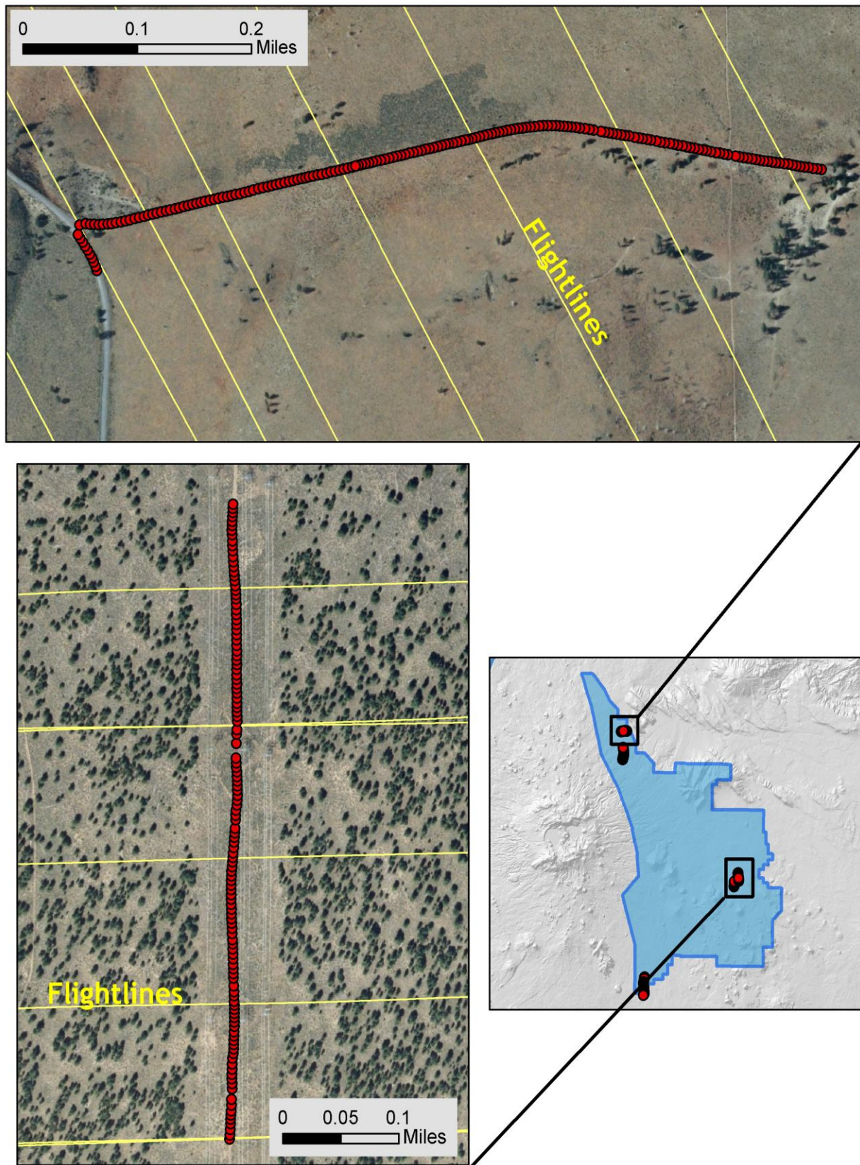
Figure 2.15. Selected RTK point locations in the study area for delivery area 15; images are NAIP orthophotos.
